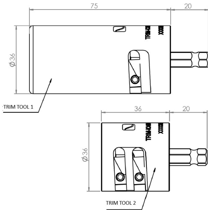
Trim Tool Outline Drawing, dimension in mm
