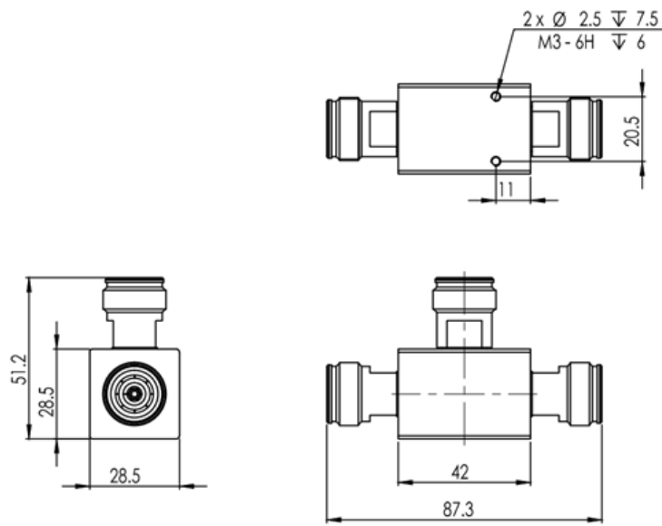
TPS5-43-555_6000_Drawing
