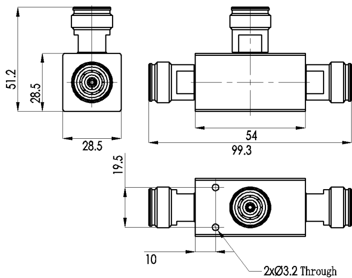
Outline Drawing
