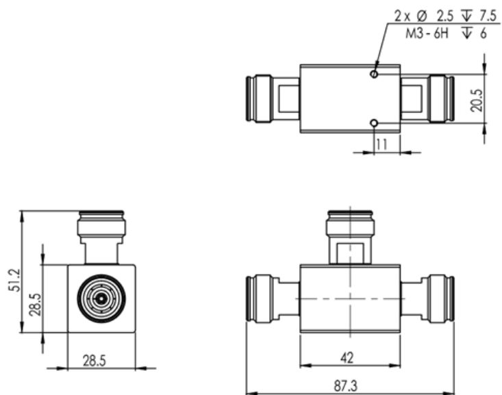
TPS10-43-555_6000_Drawing
