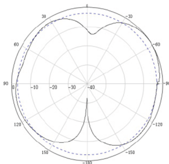
Vertical Pattern
