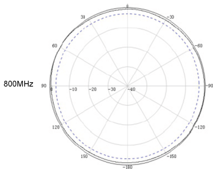
Horizontal Pattern
