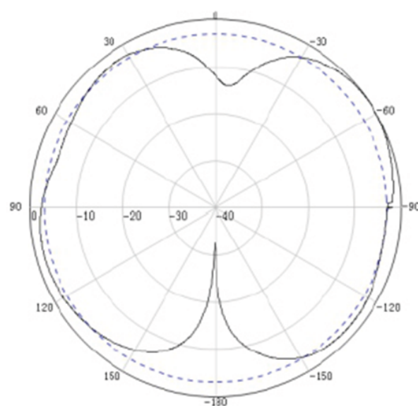
Vertical Pattern
