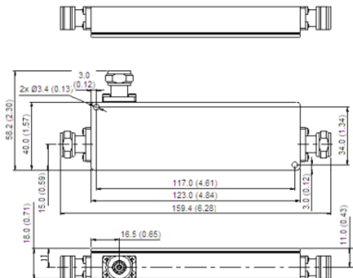
Dimensions mm(inch)
