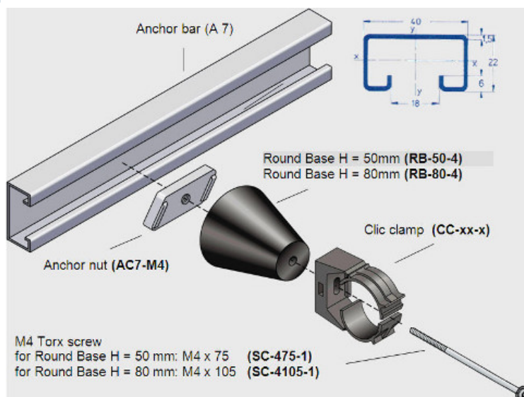
Installation example
