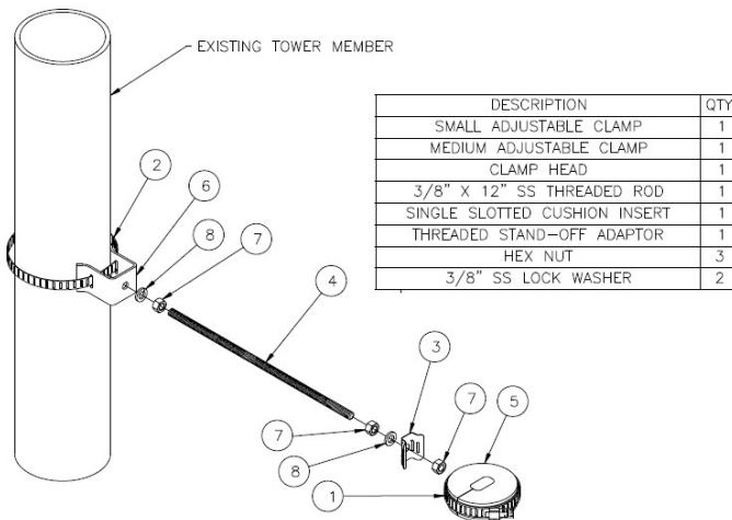
Twistflex Hanger Assembly Drawing and Parts List
