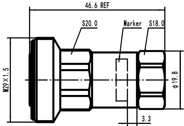
716F-SCF12-C03 Outline Drawing
