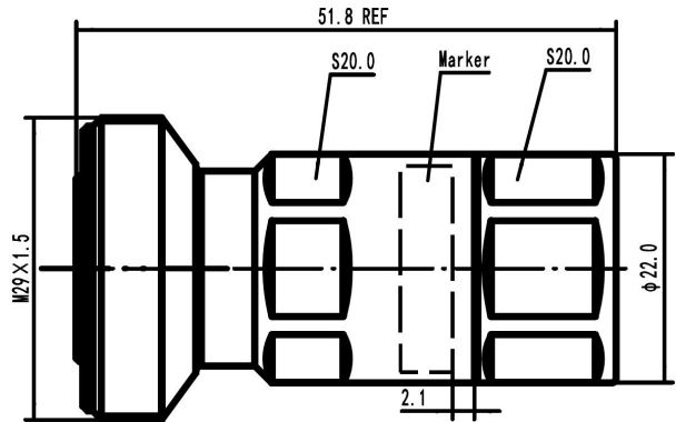
716F-LCF12-C03 Outline drawing
