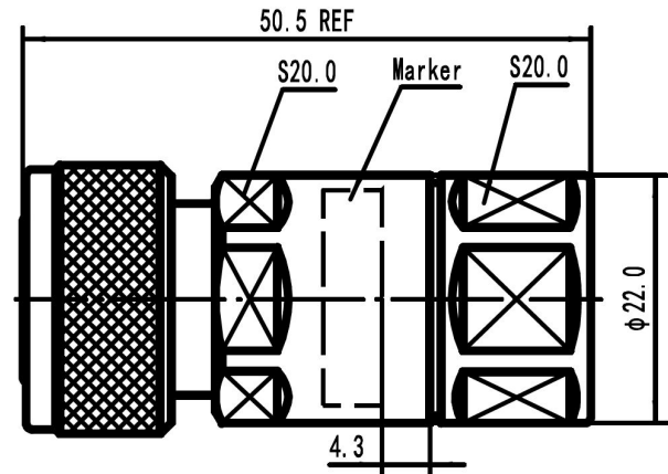
43MH-LCF12-C03 Outline drawing
