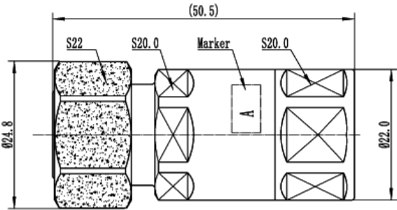
43M-LCF12-C03 Outline Drawing
