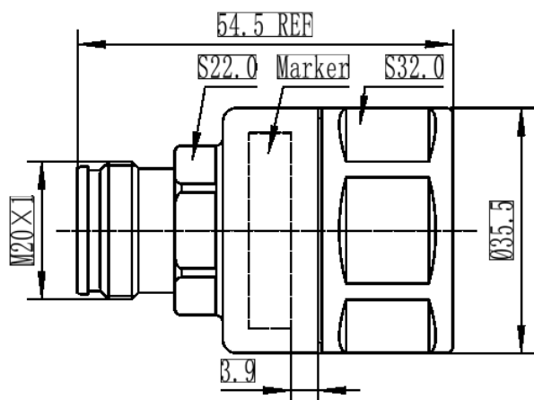
43F-LCF78-C03 Outline Drawing
