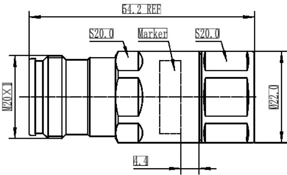
43F-LCF12-C03 Outline Drawing
