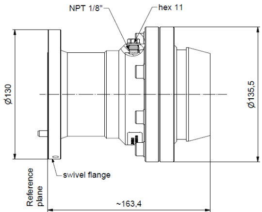
318EIA-HCA300-019 connector, dimensions in mm
